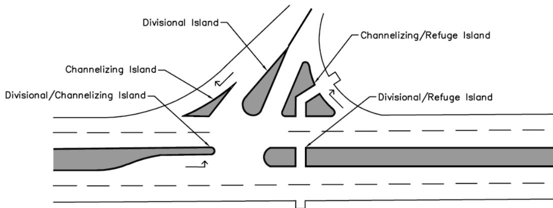
Figure 6-7. Types of Islands
