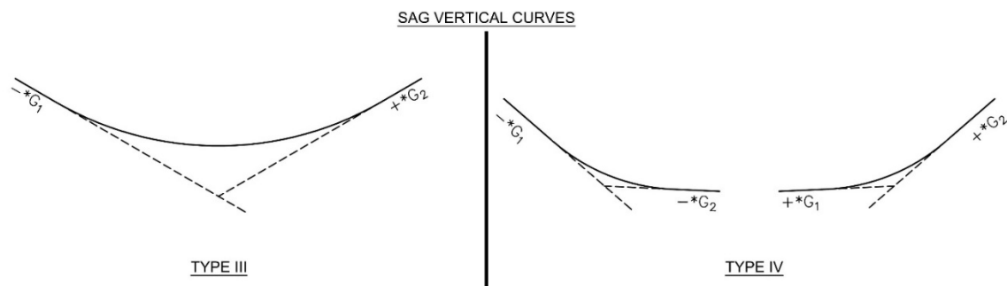
Figure 3-6. Sag Vertical Curve Types
