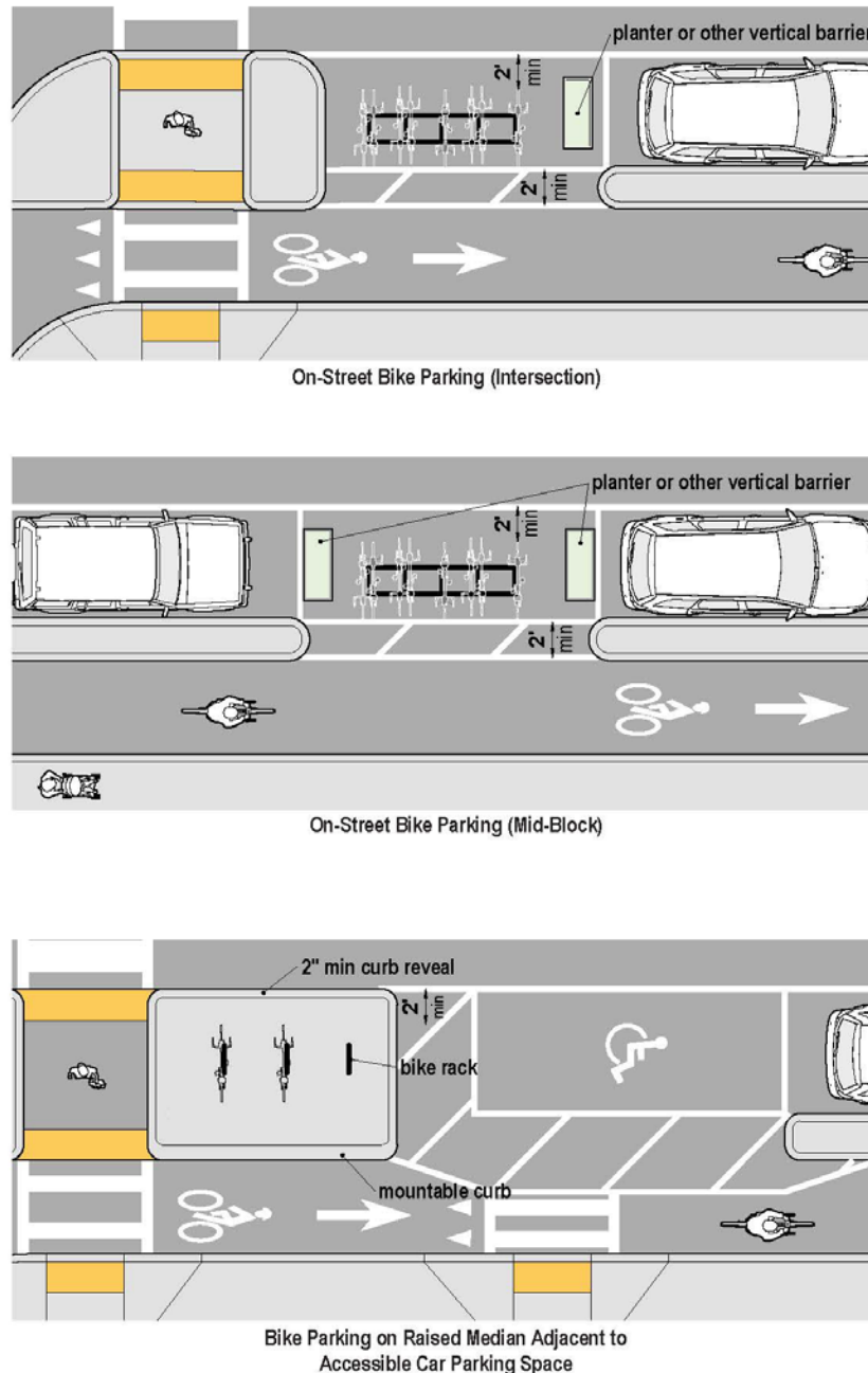
Figure 4-35. Example Designs of On-Street Bicycle Parking
