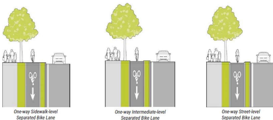
Figure 4-10. Varying Levels of One-way Separated Bicycle Lane Separation
