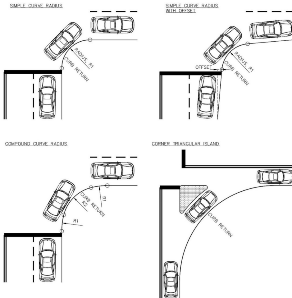
Figure 6-6. Curb Radius Design Types
