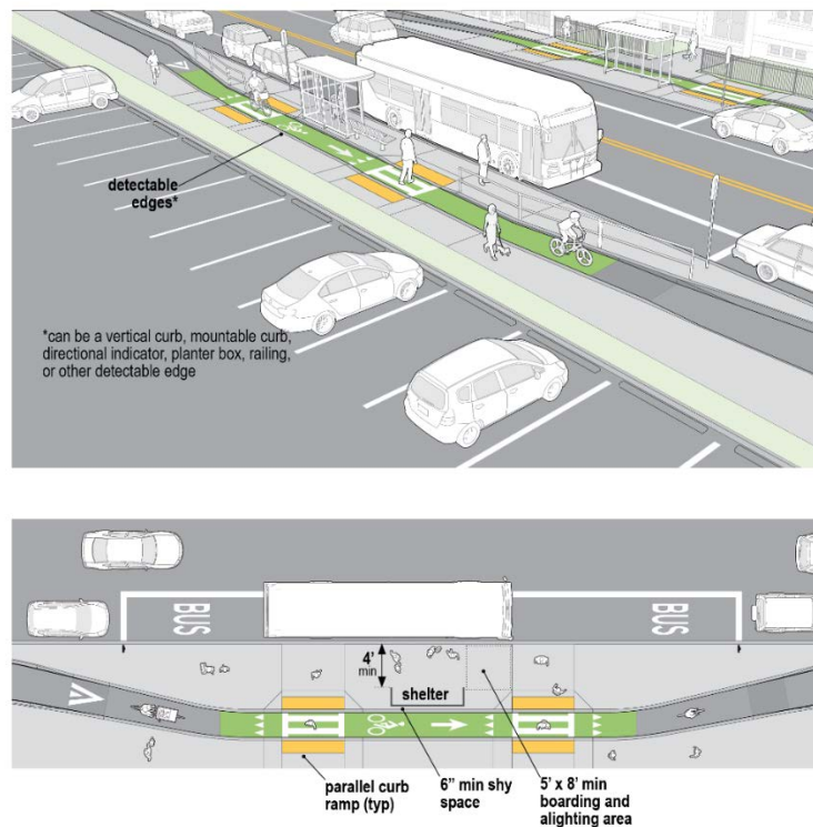
Figure 9-2. Example Separated Bike Lane at Transit Stop
