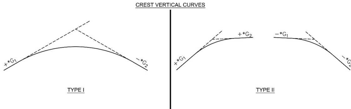
Figure 3-5. Crest Vertical Curve Types
