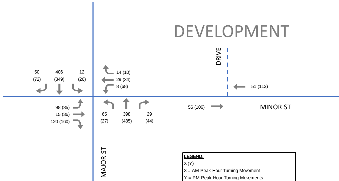
Figure 12-3. Existing Traffic Volumes Example Exhibit
