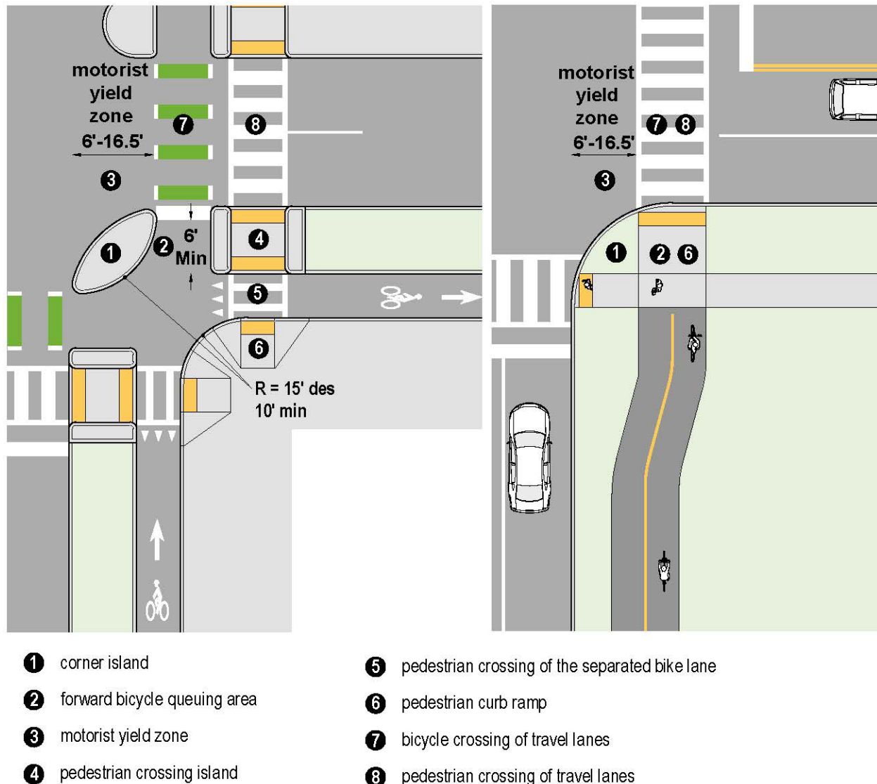
Figure 4-29. Preferred Protection Intersection Designs
