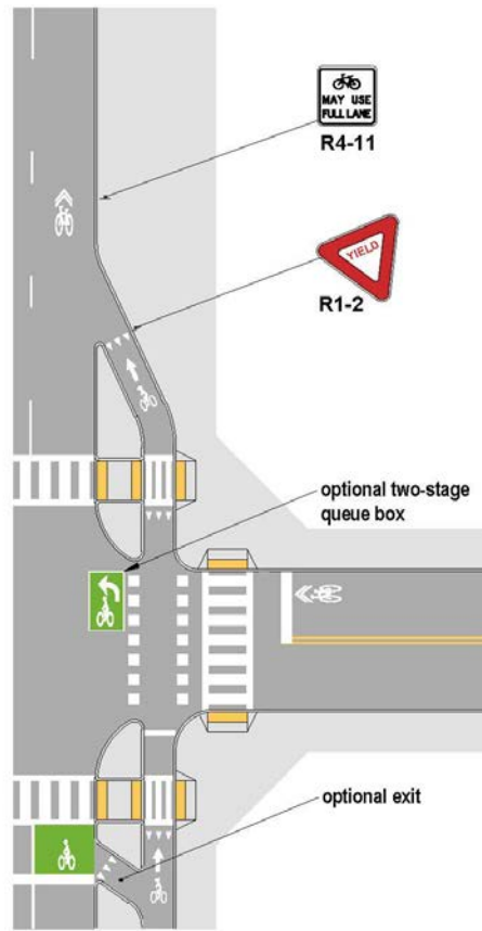
Figure 4-17. Preferred Design of a Separated Bike Lane Transition to a Shared Bike Lane
