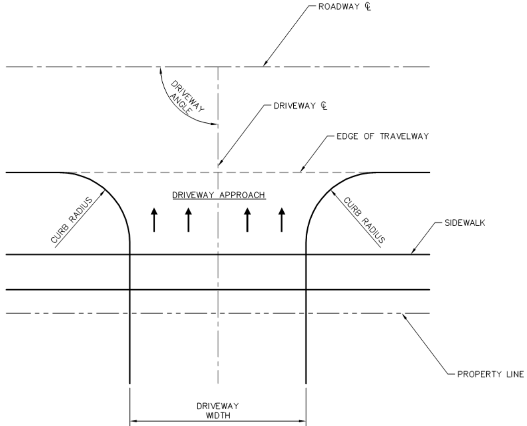
Figure 3-13. Driveway Variables
