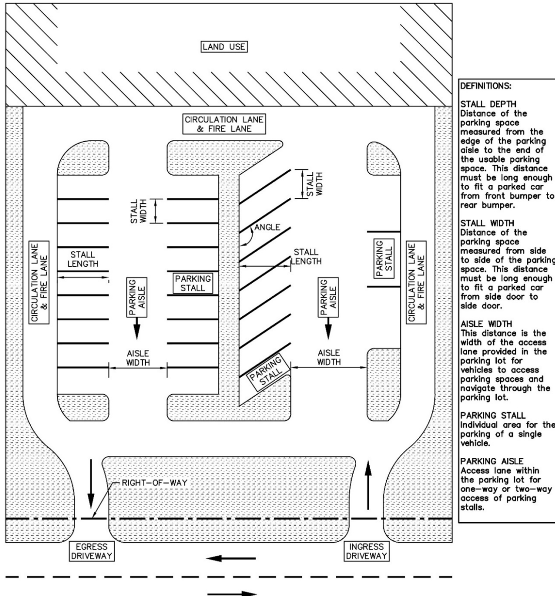
Figure 8-3. Parking Variables
