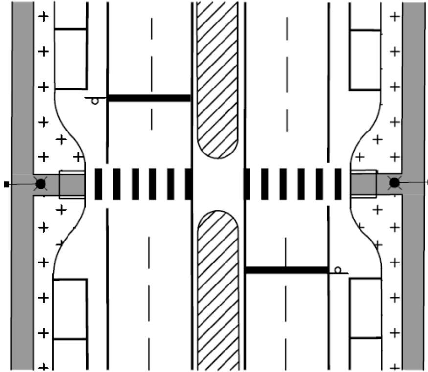
Figure 7-1. Midblock Crossing Example
