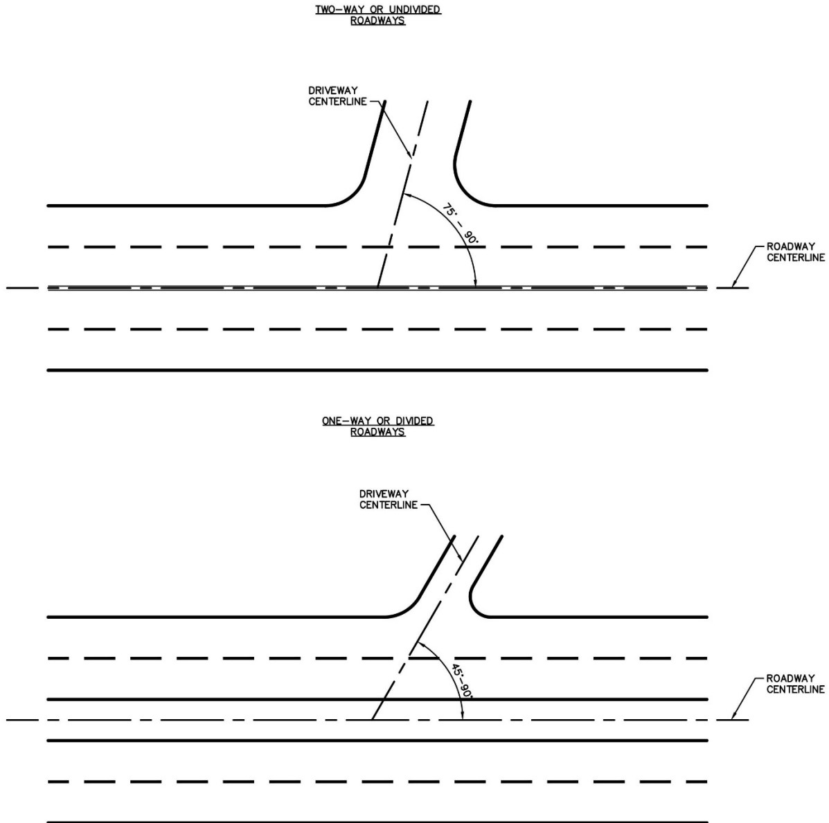
Figure 3-10. Driveway Angle
