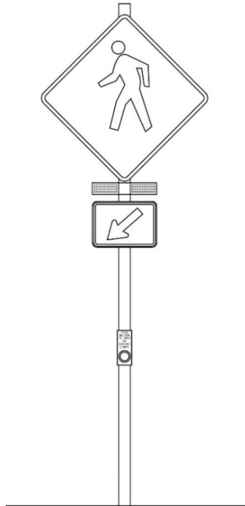
Figure 7-4. Pedestrian RRFB
