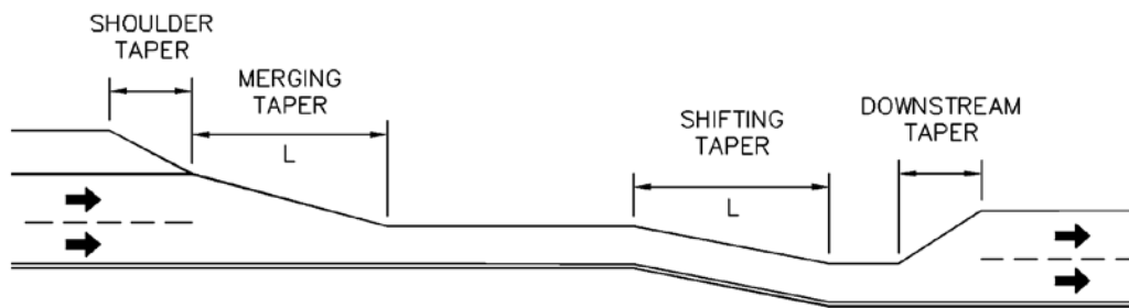
Figure 3-7. Pavement Transition Tapers
