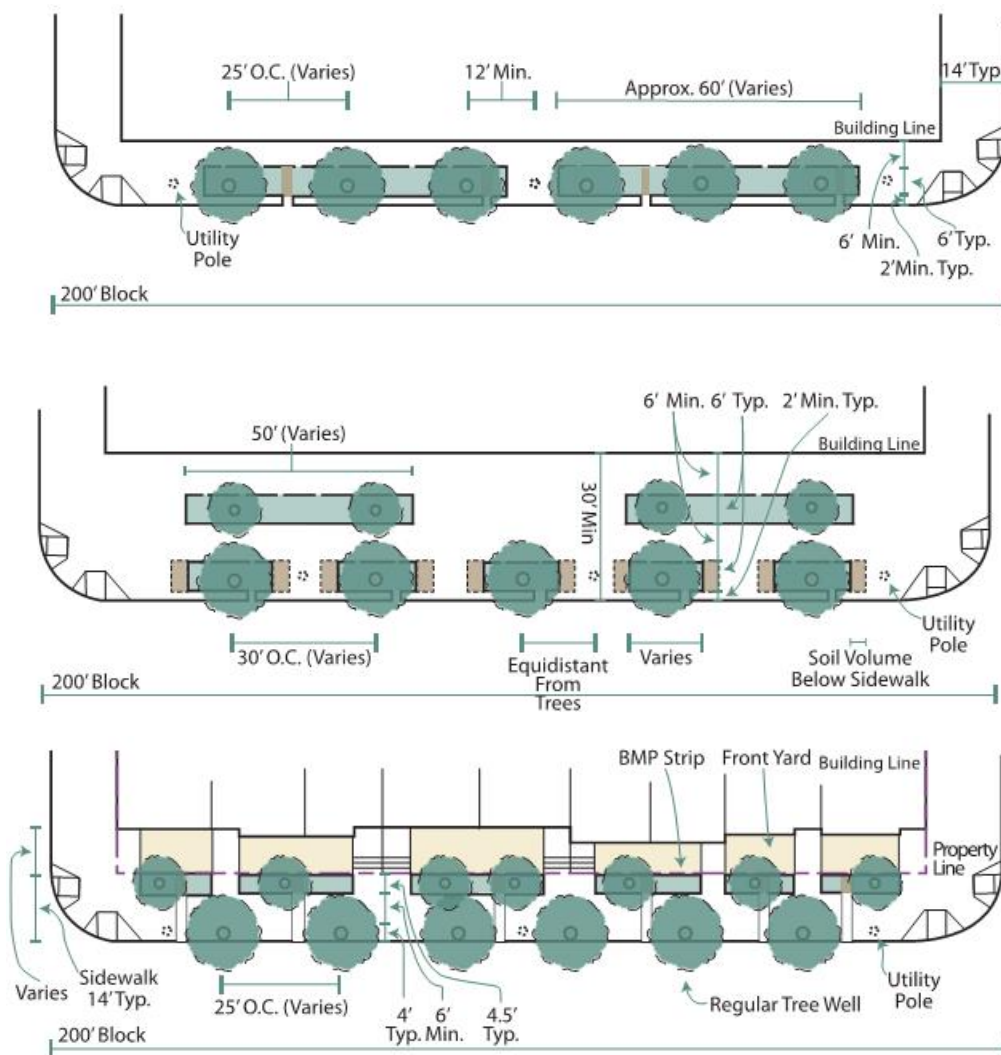
Figure 5-5. Continuous Planting Strips in the Furnishing Zone, Mid-Way, and Frontage Zone Positions
