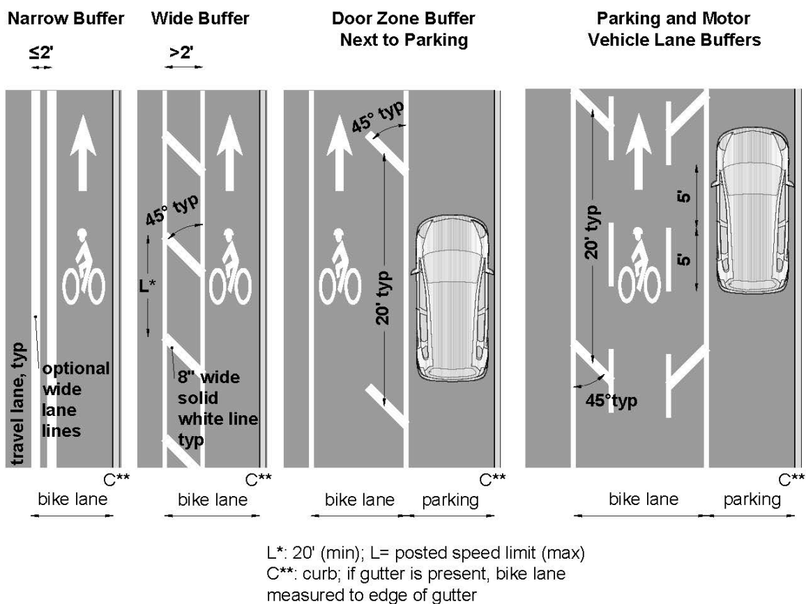
Figure 4-12. Buffered Bicycle Lane Width Guidance
