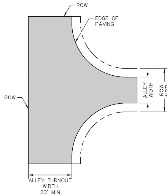
Figure 3-12. Alley Turnouts
